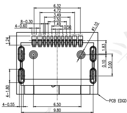
PCB LAYOUT TOLERANCE SIZE: ±0.05
