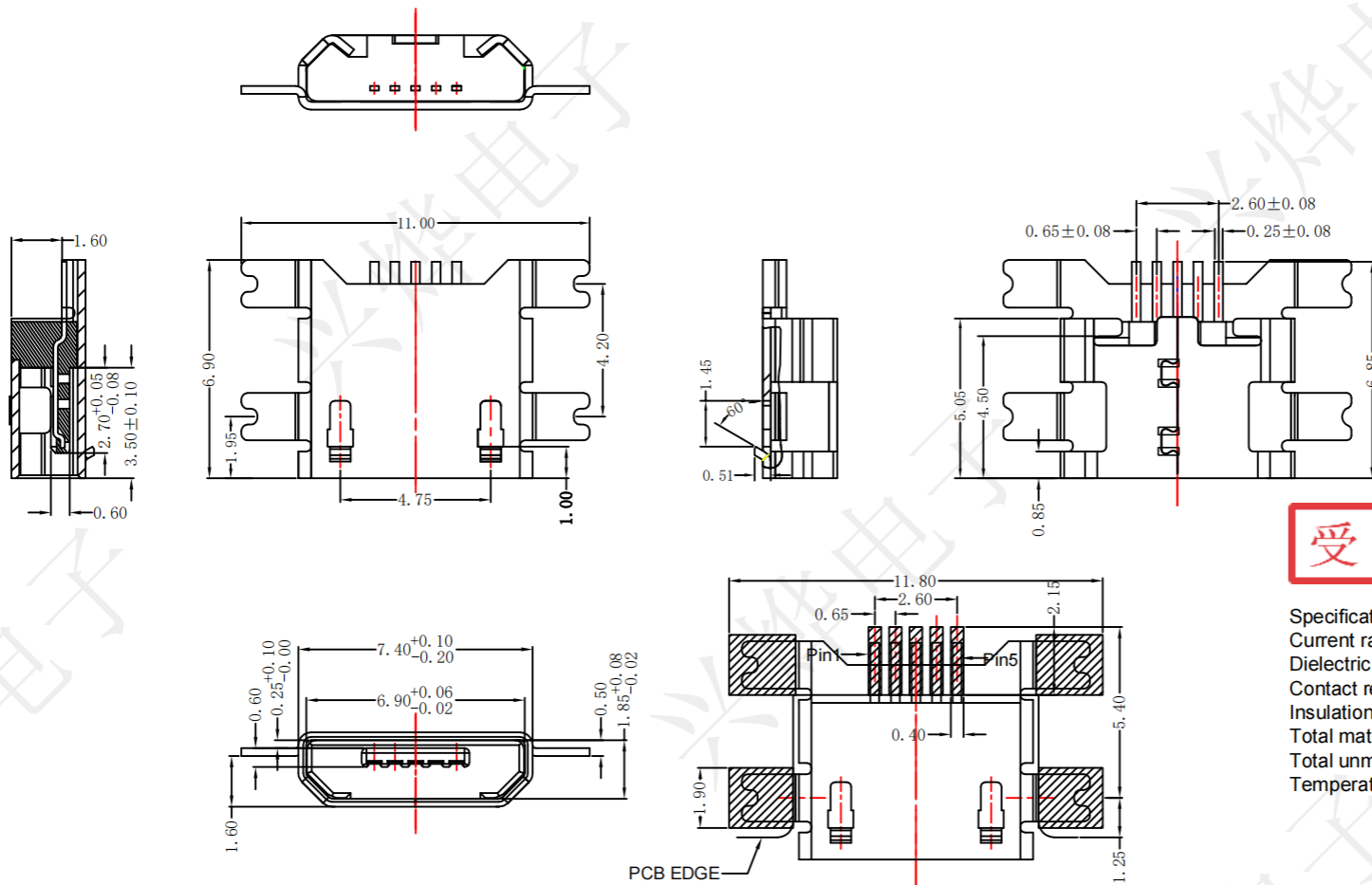
RECOMMENDED PCB LAYOUT PCB图仅供参考
