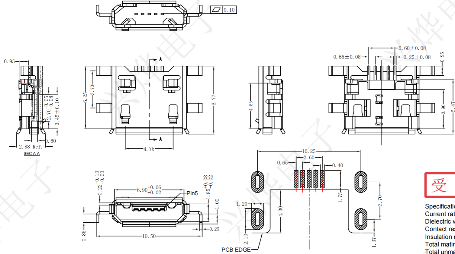
RECOMMENDED PCB LAYOUT PCB图仅供参考
