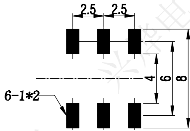
P.C.B LAYOUT DIMENSION TOP VIEW
