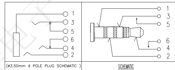
(ø3.50mm 4 POLE PLUG SCHEMATIC)
