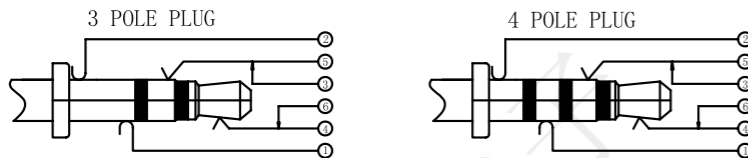
CIRCUIT DIAGRAM
